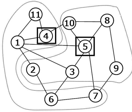
Fig. 1 Example of an unconnected territory design for p=2 and n=11 .
