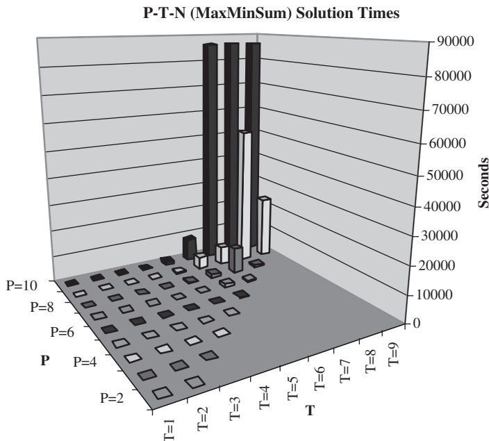
Figure 5. MaxMinSum solution times.
