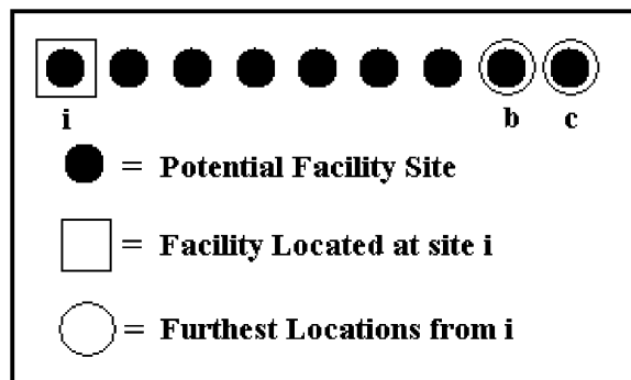
Figure 3. Linear problem demonstrating neighborhood constraint elimination.
